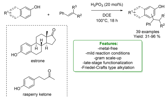
Scheme 19 H 3 PO 3 -catalysed alkylation of phenols with alkenes. 85
