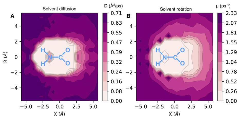
Fig. 4 Two dimensional colormaps of solvent dynamics around carbamate/carbamic acid dissolved in liquid ammonia. (A): diffusion coefficient ( D ) of N atoms in units of \text{\AA}^2 \text{ps}^{-1} . (B): N–H reorientation frequency ( \mu in units of \text{ps}^{-1} ). The 3 dimensional distribution function is projected on a molecular frame in cylindrical coordinates. The X axis corresponds to the direction along the O–C–O bisector, while the R axis is the distance from the line defined by the X axis.
