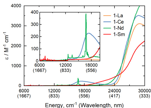
Fig. 2 UV-vis/NIR spectra of 1-Ln , 1-Ce , 1-Nd , 1-Sm , from 6000\text{--}30\,000 \text{ cm}^{-1} (inset 6000\text{--}20\,000 \text{ cm}^{-1} ) recorded as 0.5 \text{ mM} solutions in toluene at room temperature.
