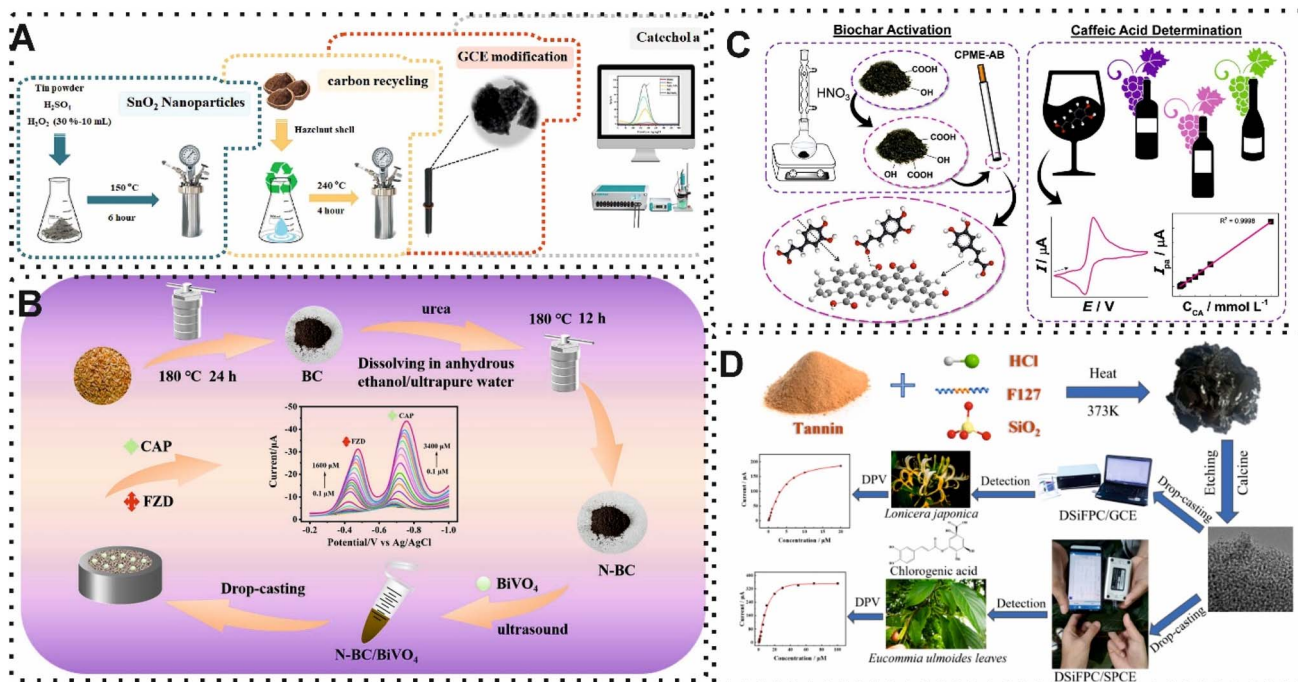
Fig. 7 (A) Representation of EC sensor which exploited carbon/ \text{SnO}_2 NPs for determination of catechol. Reproduced with permission from ref. 85. Copyright Elsevier Science, 2024. (B) Schematic of using nitrogen-BW derived carbon materials/ \text{BiVO}_4 on the surface of GCE for quantification of furazolidone and chloramphenicol. Reproduced with permission from ref. 86. Copyright Elsevier Science, 2024. (C) Illustration of the synthesized castor cake waste-derived CBMs and its application in EC sensor for caffeic acid detection. Reproduced with permission from ref. 88. Copyright Elsevier Science, 2020. (D) Schematic using carbon-based material from plant-derived tannic acid for detection of chlorogenic acid. Reproduced with permission from ref. 89. Copyright Elsevier Science, 2024.
