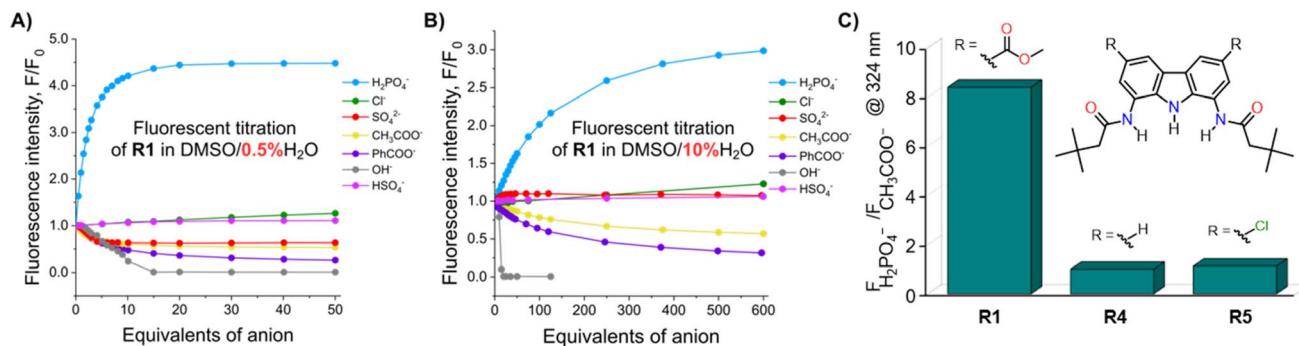
Fig. 4 The fluorescence intensity of 10 \mu\text{M} solution of R1 at 380 nm in the presence of various anions in (A) DMSO/0.5% H 2 O and (B) DMSO/10% H 2 O at 298 K. EX WL: 324 nm. (C) The fluorescence intensity ratios of phosphate and acetate complexes of receptors R1 , R4 and R5 in the presence of 50 equiv. of the anions in DMSO/0.5% H 2 O. EX WL: 324 nm, EM WL: 380 nm.
