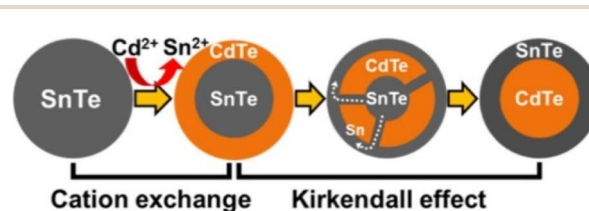
Fig. 3 Schematic illustration of the formation of SnTe-based core/shell NCs by cation exchange reaction and the Kirkendall effect. Reprinted with permission from ref. 39 Copyright (2016) American Chemical Society.
