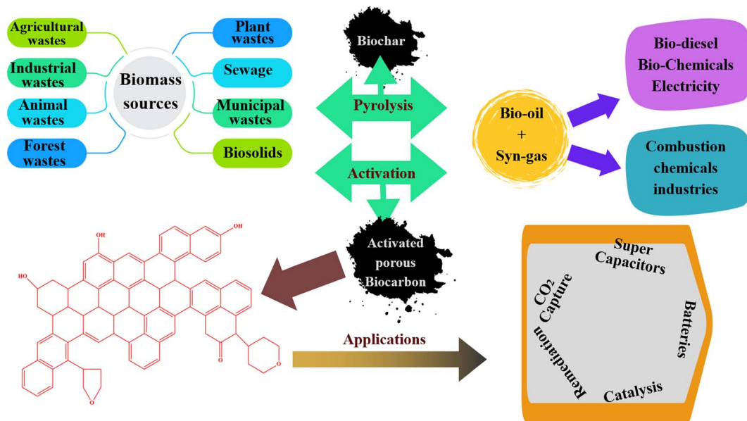
Fig. 2 Illustration of the process of producing biochar and activated carbons from biomass together with their potential applications across different industries. Reproduced from ref. 11.
