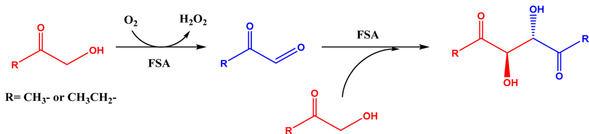
Fig. 5 Aldol reaction of hydroxyketones catalyzed by \beta -fructose-6-phosphate aldolase (FSA).
