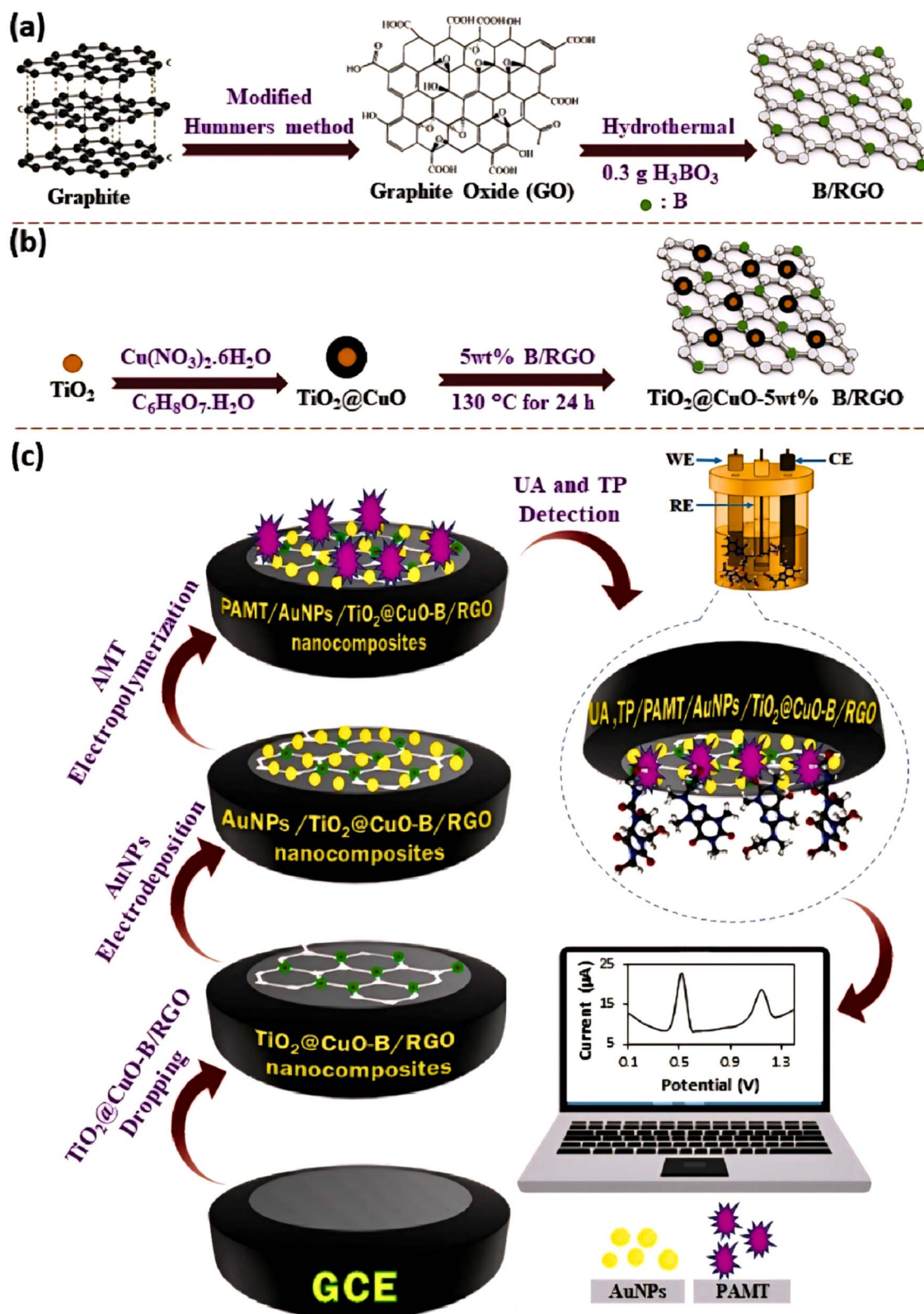
Fig. 3 Procedure for the preparation of (a) B/RGO nano-sheet, (b) \text{TiO}_2 @ \text{CuO} \text{-} \text{B/RGO} nanocomposites, and (c) design of electrochemical sensor for the simultaneous detection of UA and TP by the \text{PAMT} / \text{AuNPs} / \text{TiO}_2 @ \text{CuO} \text{-} \text{B/RGO} nanocomposite. Reprinted with permission from ref. 117. Copyright (2023), Elsevier.
