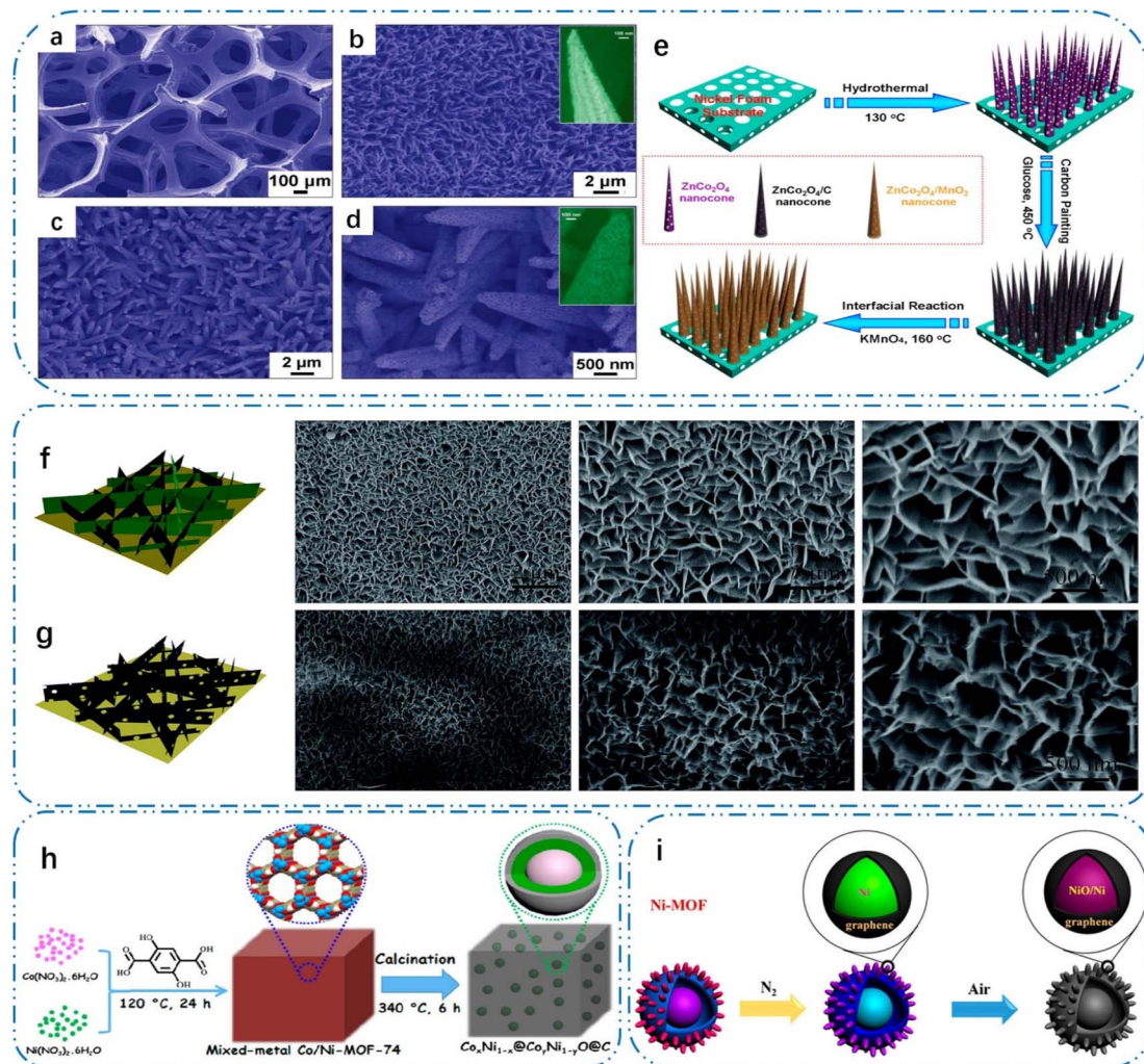
Fig. 6 SEM images of (a) Ni foam; (b) ZnCo 2 O 4 NCFs (and a magnified view in inset); (c) and (d) ZnCo 2 O 4 /MnO 2 NCFs taken at different magnifications. (e) Schematic illustration of the fabrication processes of ZnCo 2 O 4 /MnO 2 composite nanocone forests (NCFs) with a hierarchical core/shell structure, reproduced from ref. 11 with permission from [Elsevier], Copyright [2015]. Schematic illustration and SEM images of (f) ultrathin Ni 3 (NO 3 ) 2 (OH) 4 nanoflakes and (g) ultrathin porous NiO nanoflakes on nickel foam at different magnifications, reproduced from ref. 18 with permission from [the Royal Society of Chemistry], Copyright [2016]. (h) Illustration of the synthetic scheme for Co x Ni 1-x @Co y Ni 1-y O@C, reproduced from ref. 30 with permission from [the American Chemical Society], Copyright [2017]. (i) Schematic illustration of the formation of NiO/Ni/graphene composites, reproduced from ref. 37 with permission from [the American Chemical Society], Copyright [2016].
