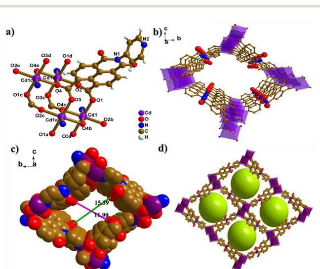
Fig. 1 Crystal structure of CdPNMI. (a) Representation of the Cd coordination environment; (b) 3D net with abundant nitrogen and oxygen sites along the inner channel walls; (c) space-filling model of a 1D channel viewed along the a -axis; (d) view of 1D channels along the a axis filled with green balls.
