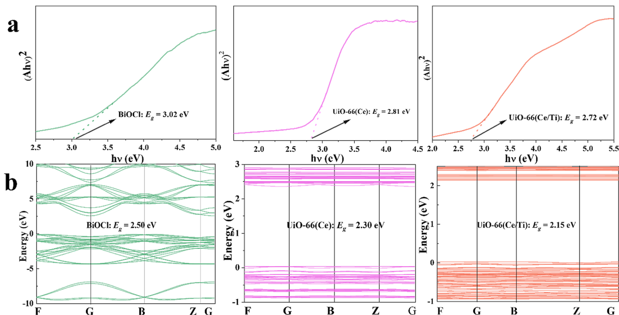
Fig. 3 (a) Plots of (\text{Ah}\nu)^{1/2} or (\text{Ah}\nu)^2 vs. h\nu for the band gap energy of the samples calculated using the Kubelka–Munk function formula. (b) Band structures of the samples calculated by DFT simulations.
