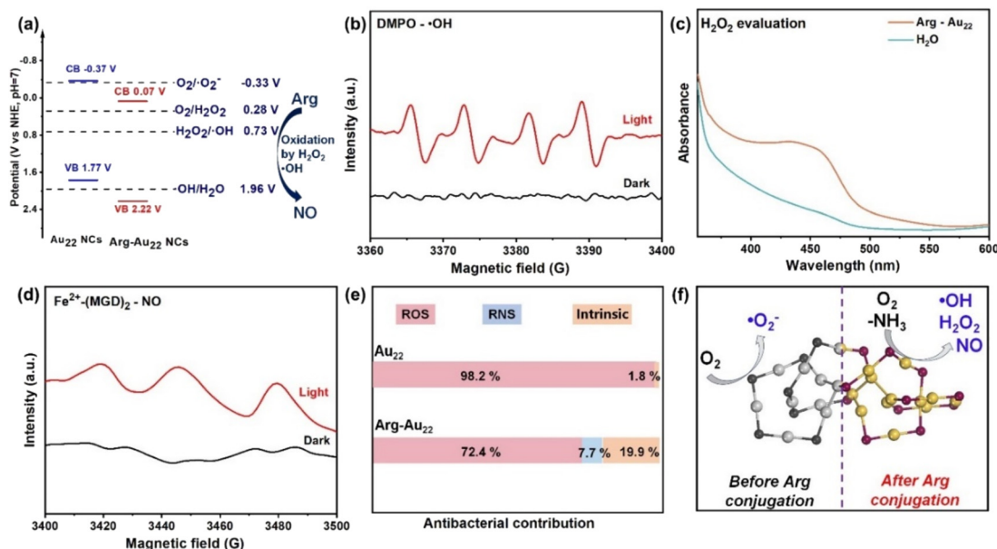
Fig. 3 (a) Energy level diagram of Arg-Au 22 and pristine Au 22 NCs. (b) EPR spectra of • OH of the Arg-Au 22 NCs with or without visible light illumination. (c) Absorbance of the generated H 2 O 2 over Arg-Au 22 NCs under visible light illumination and bubbling O 2 for 60 min. (d) EPR spectra of NO of the Arg-Au 22 NCs with or without visible light illumination. (e) Specific antibacterial contributions of ROS, RNS and intrinsic antibacterial Au species over Arg-Au 22 and pristine Au 22 NCs. (f) Schematic illustration of the photodynamic ROS/RNS production modality of Au 22 NCs before and after Arg conjugation.
