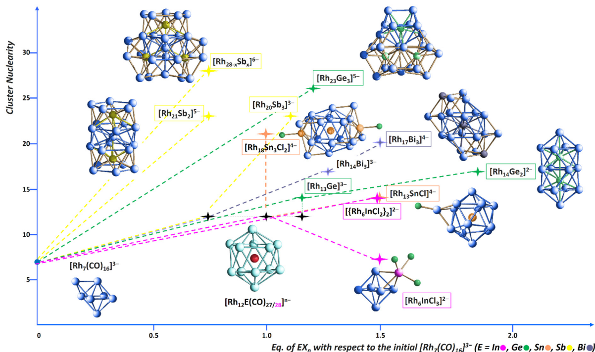
Fig. 9 Growth trend of heterometallic carbonyl clusters for the various Rh–E systems as a function of the added equivalents of EX_n ( X = \text{Cl, Br; } n = 2\text{--}4 ). Carbonyl ligands have been omitted in the stated formulas, for sake of clarity. Rh atoms are depicted in blue, in magenta, Ge in bright green, Sn in orange, Sb in yellow, Bi in violet.
