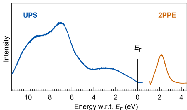
Fig. 7 (bottom) UPS and 2PPE spectra of a thick Ta@Si 16 SA film (7 MLs). The energy onset at E_F in the UPS spectrum indicates the ohmic electronic conduction of the Ta@Si 16 SA film. The broad valence and conduction band features, E_F - 2.6 eV, -7.0 eV, and -9.6 eV in UPS and E_F + 2.1 eV in 2PPE, are observed. The experimental results are compared with DFT calculations for the geometric isomer of neutral species and cations, as shown ESI Fig. S8.†
