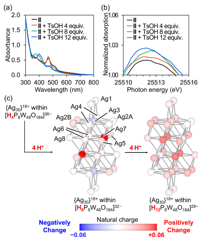
Fig. 4 (a) UV–vis spectra of II after adding TsOH (4, 8, and 12 equivalents) in acetonitrile. (b) The enlarged view around the white line ( E \approx 25\,512 eV) of solution-state Ag K-edge XANES spectra of II upon TsOH addition in acetonitrile. (c) Changes in the natural charge of the \{\text{Ag}_{30}\}^{18+} nanocluster within a ring-shaped POM upon protonation. Change in the natural charge of each Ag atom after adding protons to a ring-shaped POM framework. Ag atoms are color-coded based on the changes in the natural charges.
