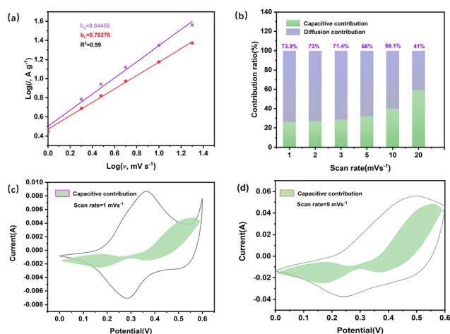
Fig. 8 (a) Kinetic characteristics and reaction mechanism of \text{CoNi}_{0.5}\text{-MOF/CC} electrode; (b) the capacitive contribution of \text{CoNi}_{0.5}\text{-MOF/CC} at different scan rates; (c and d) the capacitive contribution at 1 \text{mV s}^{-1} and 5 \text{mV s}^{-1} .
