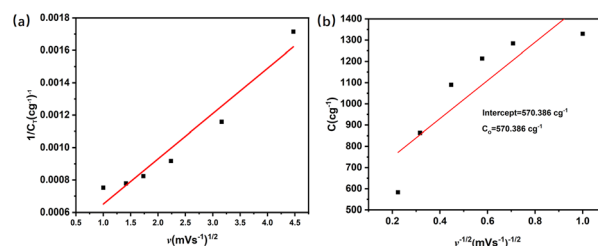
Fig. 9 Kinetic characteristics and reaction mechanism of \text{CoNi}_{0.5}\text{-MOF/CC} electrode: (a) fitting theoretical capacity; (b) fitting theoretical capacitive capacity (Trasatti's method).
