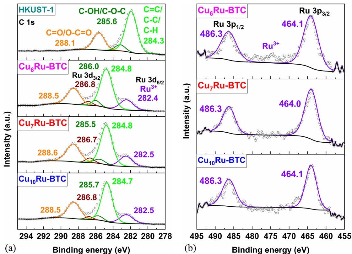
Fig. 5 HR-XPS spectra of (a) C 1s and Ru 3d and (b) Ru 3p for \text{Cu}_{10}\text{Ru-BTC} , \text{Cu}_7\text{Ru-BTC} , \text{Cu}_6\text{Ru-BTC} and mechanochemically synthesized HKUST-1.
