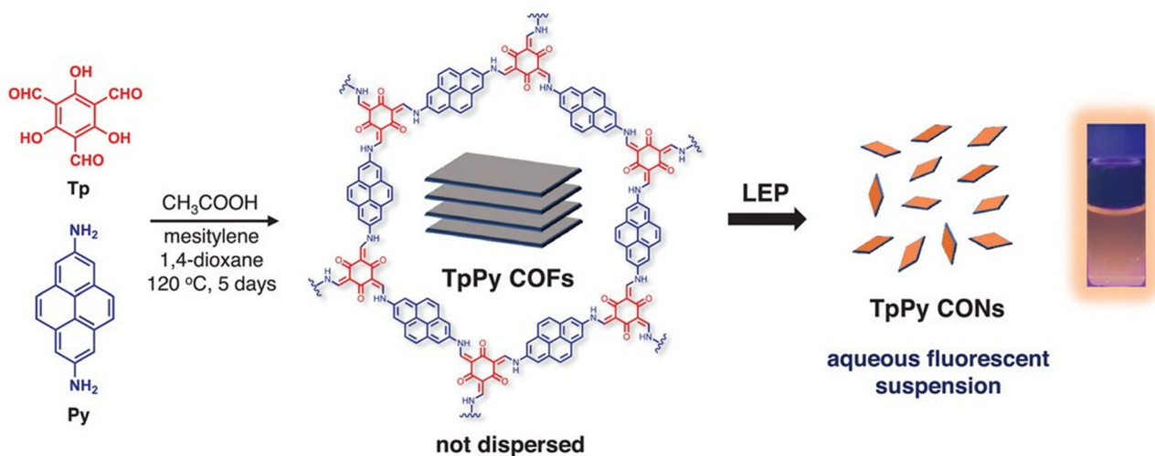
Fig. 2 Schematic diagram of the preparation of TpPy CONs by solvothermal condensation and liquid exfoliation process (fluorescent photograph of a 0.5\text{ mg mL}^{-1} TpPy CON dispersion taken under 365\text{ nm} UV light). Adapted with permission from ref.79.
