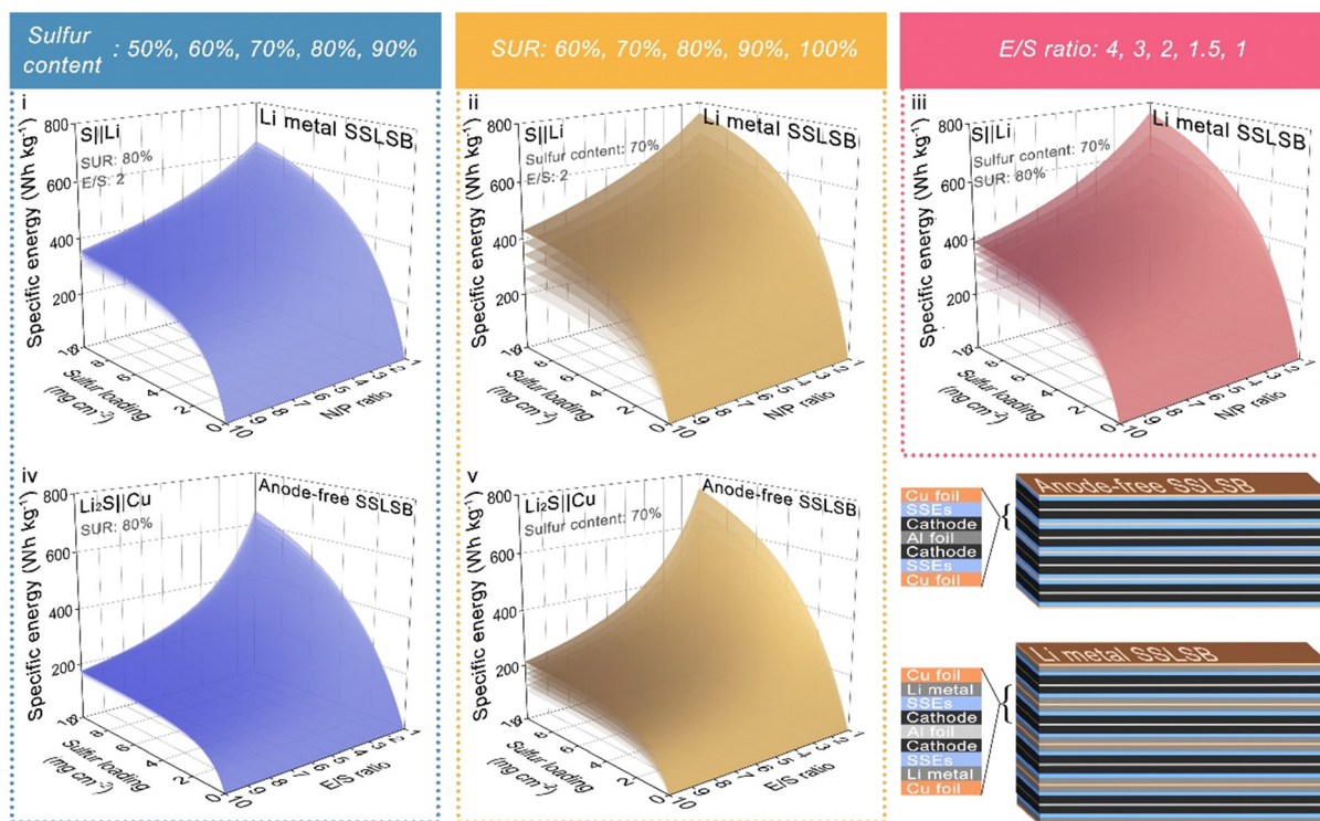
Fig. 3 The energy density of SSLSB (S||Li top, \text{Li}_2\text{S}||\text{Cu} bottom) in terms of various sulfur loading, sulfur content, sulfur utilization ratio, E/S ratio, and N/P ratio and the schematic of stacked SSLSBs based on S||Li and \text{Li}_2\text{S}||\text{Cu} .
