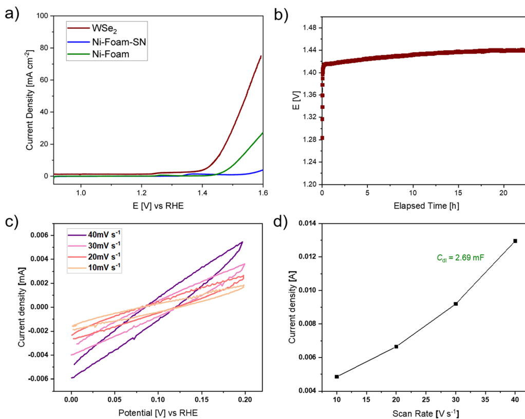
Fig. 6 (a) Linear sweep voltammetry of WSe 2 flower-like structures with Super P ® Li and Nafion on nickel foam (WSe 2 , red curve) in comparison to only Super P ® Li and Nafion on nickel foam (Ni-foam-SN, blue curve) and bare nickel foam (Ni-foam, green curve) used as references (b) chronopotentiometry of WSe 2 at a current density of 10 mA cm -2 , (c) cyclic voltammetry curves at different scan rates from 10–40 mV s -1 and (d) current density vs. scan rate for calculation of the double-layer capacitance ( C_{dl} = 2.69 mF).
