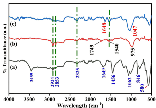
Fig. 2 FTIR analysis of different electrodes: (a) SPE, (b) anti-CYFRA21-1/SPE, and (c) anti-TP53/SPE immunoplatfoms.
