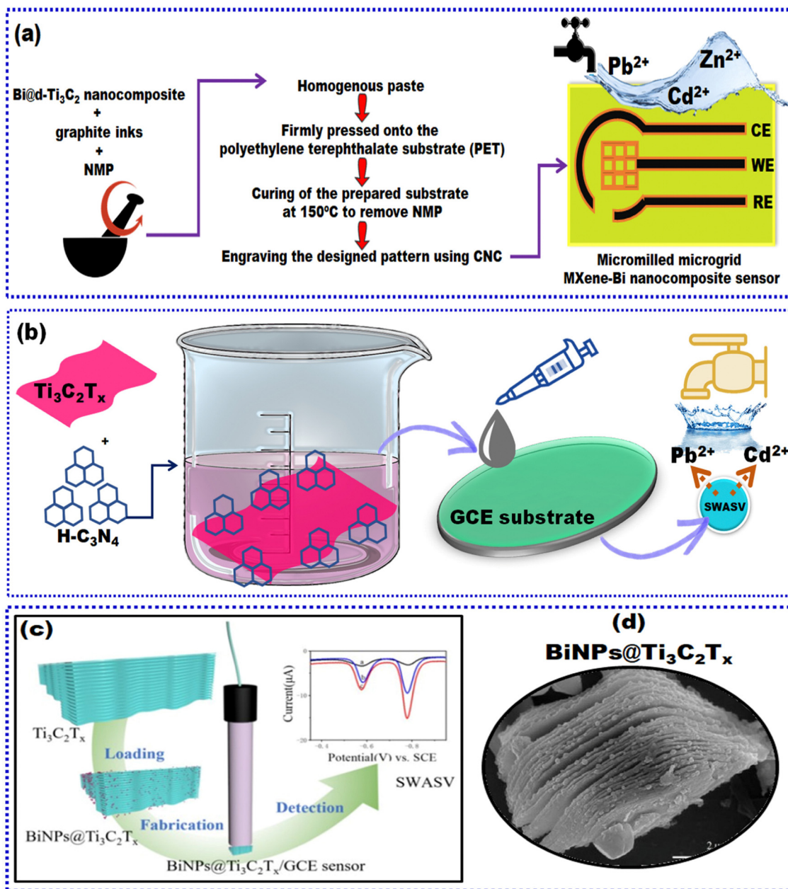
Fig. 9 (a) Construction scheme for Bi@ \text{Ti}_3\text{C}_2\text{T}_x /MSE and (b) schematic representation of \text{H-C}_3\text{N}_4/\text{Ti}_3\text{C}_2\text{T}_x synthesis, and fabrication of \text{C}_3\text{N}_4/\text{Ti}_3\text{C}_2\text{T}_x /GCE. (c) Graphical illustration of BiNPs@ \text{Ti}_3\text{C}_2\text{T}_x /GCE sensor construction and (d) TEM image of BiNPs@ \text{Ti}_3\text{C}_2\text{T}_x . 171 Reproduced with permission from ref. 171. Open access MDPI (2020).
