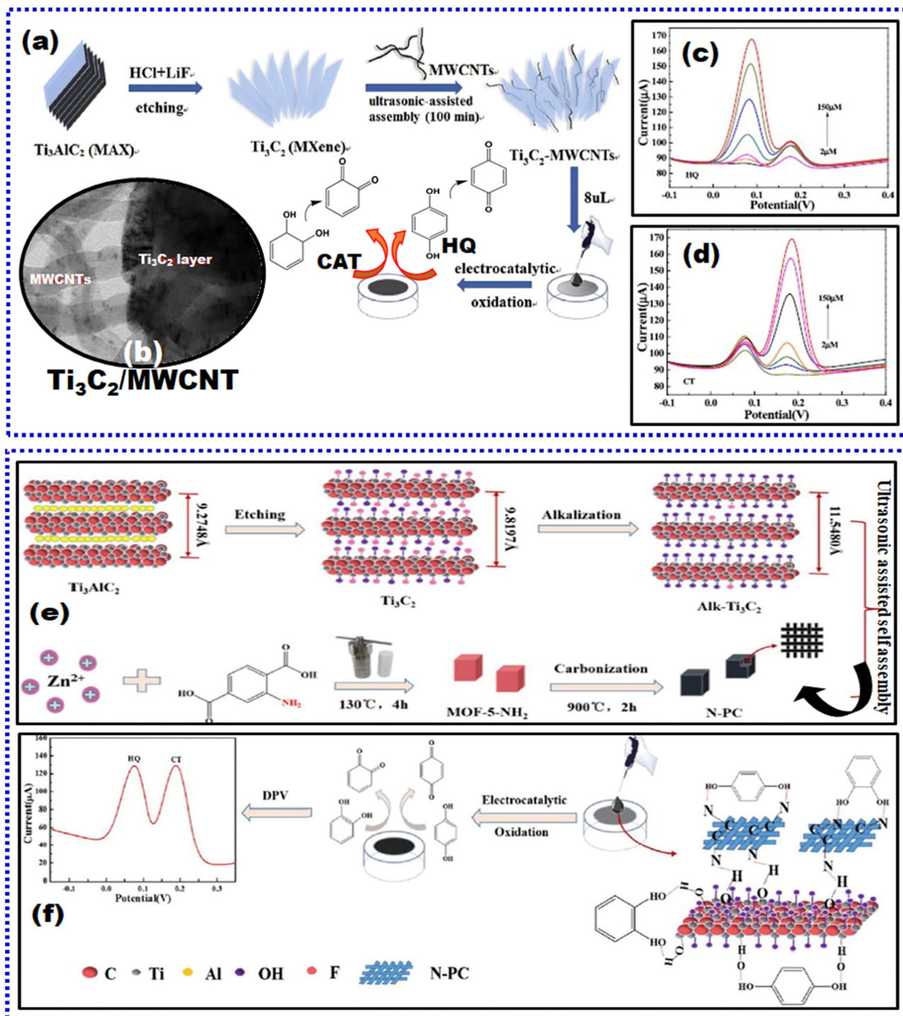
Fig. 13 (a) Schematics of \text{Ti}_3\text{C}_2/\text{MWCNT} synthesis and fabrication of the EC sensor for CAT and HQ oxidative quantification. (b) TEM image of \text{Ti}_3\text{C}_2/\text{MWCNT} s and DPV signal for (c) HQ and (d) CAT at various concentrations. 195 (e) Schematic of \text{Alk-Ti}_3\text{C}_2/\text{N-PC} composite synthesis. (f) Graphical representation of \text{Alk-Ti}_3\text{C}_2/\text{N-PC}/\text{GCE} sensor fabrication and the response of CAT and HQ oxidation process. 196 Reproduced with permission from ref. 195, and 196. Copyright Elsevier (2019), and Elsevier (2020).
