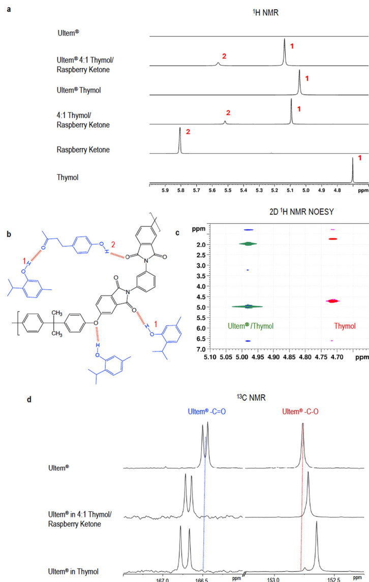
Fig. 3 NMR spectroscopy analysis of Ultem ^{\circledR} solutions. (a) ^1\text{H} NMR spectra of different solutions and individual components. (b) Hydrogen bond structures between Ultem ^{\circledR} , thymol and raspberry ketone. (c) 2D ^1\text{H} NMR NOESY overlap spectra of thymol and Ultem ^{\circledR} /thymol. (d) ^{13}\text{C} NMR spectra of Ultem ^{\circledR} and its solutions in thymol and in 4 : 1 thymol/raspberry ketone.
