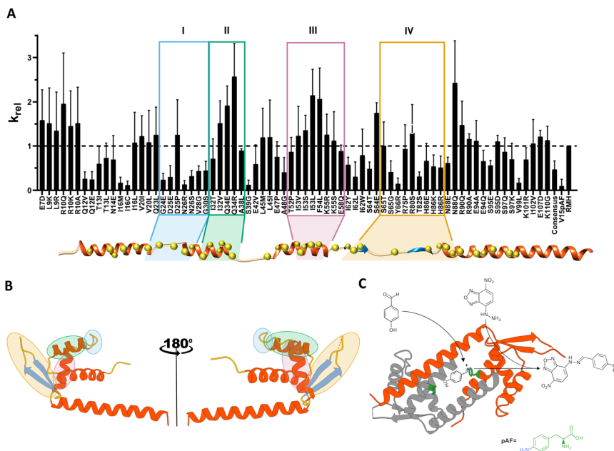
Fig. 1 (A) Relative activity profile observed for the predicted mutants in cell lysate screening. The screening was performed with 50 \mu\text{M} NBD-H, 5 mM 4-HBA in buffer R, pH 7.5, 5% DMF at 25 ^{\circ}\text{C} . The error bars represent the standard deviation of three independent measurements. Four groups of residues (clusters I, II, III and IV) with similar behaviour are marked in different colours (cyan, green, magenta, yellow) and illustrated over the LmrR secondary structure. Yellow spheres represent the positions selected for mutagenesis. (B) The four clusters identified are represented over the LmrR tertiary structure. (C) Hydrazone formation reaction scheme between 4-HBA and NBD-H. The iminium ion intermediate is represented bound to the catalytic ncAA pAF (green).
