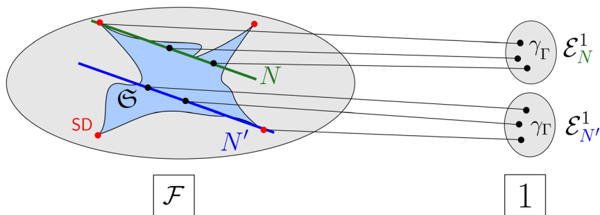
Fig. 3 Illustration of the one-to-one relation between the set \mathcal{S} (light blue) of free states on the Fock space \mathcal{F} (gray) and the sets of 1RDMs \mathcal{E}_N^1 for two different particle numbers N, N' . The red dots illustrate its extremal elements, which are the Slater determinants. For fixed particle number N , the free states \Gamma corresponding to 1RDMs \gamma_\Gamma \in \mathcal{E}_N^1 lie on a hyperplane with average particle number \langle \hat{N} \rangle_\Gamma = N .
