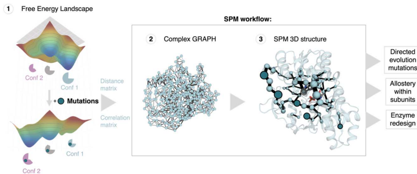
Fig. 1 Shortest path map (SPM) construction, workflow and applications. SPM is a correlation-based tool that can be used to identify conformationally relevant positions of importance for inducing a population shift in the FEL. The first step requires the estimation of the conformational heterogeneity of the studied system (FEL estimation) using for instance MD simulations. From these simulations the distance and correlation matrices are constructed, which are used to generate a first complex graph (shown in step 2, middle panel) that contains all protein residues represented as spheres and some edges of different length (weighted according to the correlation value) that link those positions situated, on average, less than 6 Å along the MD run. This complex graph is further simplified by finding the edges that are shorter, i.e. , more correlated, providing the final SPM graph than can be plotted on top of the 3D structure (step 3). In the SPM graph, the sphere size and edges are weighted according to the number of times the pair of residues have been included in the shortest paths ( i.e. , the size qualitatively represents the importance of the identified positions for the conformational dynamics of the enzyme). SPM has been used to rationalise DE mutations, 11 to study and understand the allosteric regulation within monomers in multimers, 12,15 and more recently to design new enzyme variants starting from natural scaffolds. 14,15 SPM is a strategy to reduce the number of potential hotspots, thus reducing the sequence space for enzyme engineering. The figure has been generated with a model system, the SPM graph, and displayed structure correspond to the beta subunit of tryptophan synthase.
