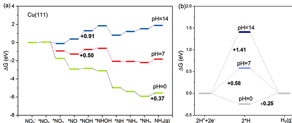
Fig. 4 The competition between (a) \text{NO}_3\text{RR} and (b) HER on Cu (111) at pH = 0, 7 and 14, studied by Hu et al. Reprinted with permission from ref. 33. Copyright 2021, American Chemical Society.
