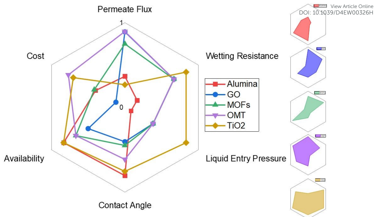
Fig. 9 Outline comparison of selected fillers used in membrane distillation.
