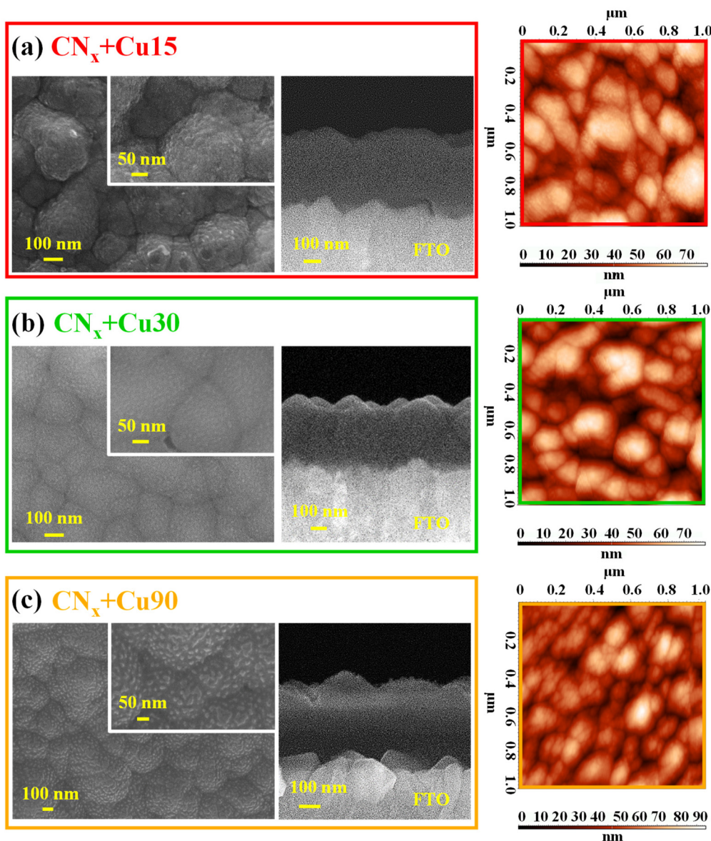
Fig. 6 Representative plane-view (left panel) and cross-sectional (central panel) FE-SEM images for the \text{CN}_x + \text{Cu15} (a), \text{CN}_x + \text{Cu30} (b), \text{CN}_x + \text{Cu90} (c). Right panel: AFM micrographs for the same specimens.
