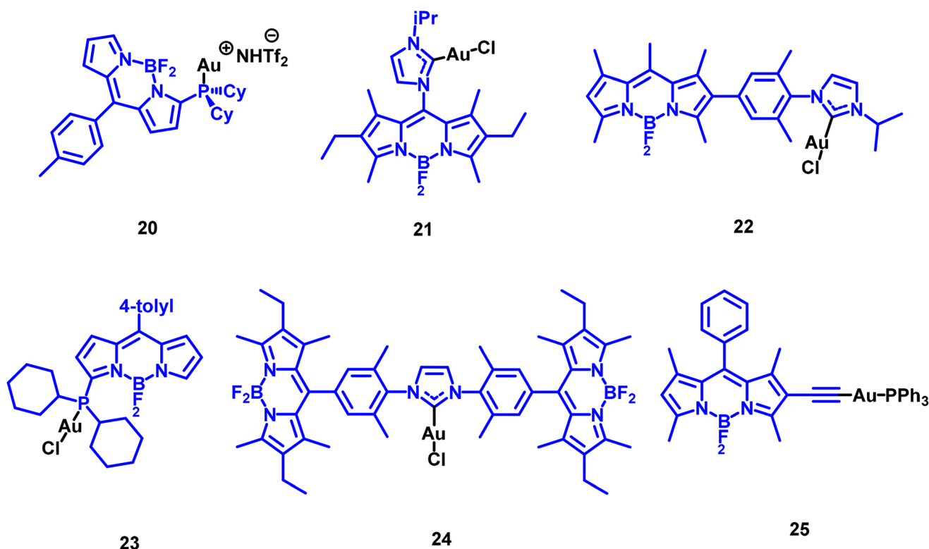
Fig. 7 Gold(I) complexes containing BODIPY ligands studied as PS.
