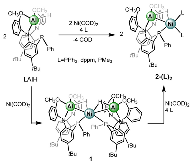
Scheme 2 Synthesis of complexes 2-(L) 2 .
