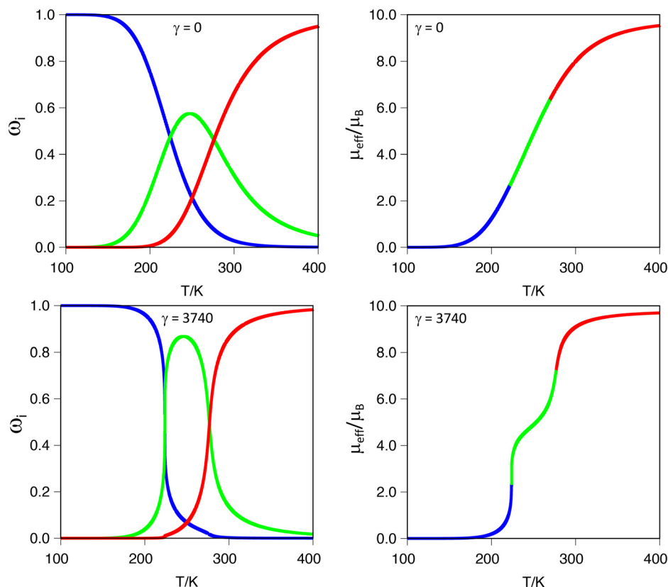
Fig. 4 (Left) Spin state populations ( \omega_i ) for the [(\text{Fe}_2(\text{L}_1)_3)@\text{Cl}]^{3+} systems with \gamma = 0 (top) and \gamma = 3740 (bottom): i = [\text{LS}-\text{LS}] (blue), [\text{HS}-\text{LS}] (green) and [\text{HS}-\text{HS}] (red) populations. (Right) Estimation of the magnetic moment computed from the corresponding spin-state populations. \gamma in \text{J mol}^{-1} .
