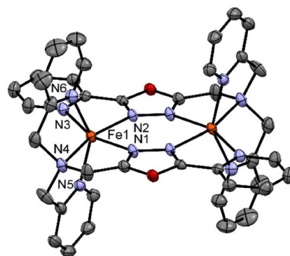
Fig. 4 Crystal structure of the complex [\text{Fe}_2^{\text{II}}(\text{L}^{\text{TetraPy}})](\text{ClO}_4)_4 \cdot \text{CH}_3\text{NO}_2 \cdot 1.5 \text{ H}_2\text{O} at 150 K. Hydrogen atom and counter ions and solvent molecules are omitted for clarity.
