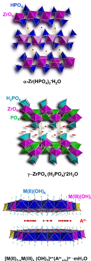
Fig. 2 Schematic view of \alpha -ZrP, \gamma -ZrP and LDHs structures.
