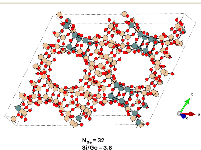
Fig. 6 The global structure optimum for the UTL system with \text{Si/Ge} = 3.8 adopting a large simulation cell (Table S4†) – compare with Fig. 4. The Ge content at this Si/Ge ratio allows for a complete filling of D4R units with germanium atoms, however, a partial spillover of Ge atoms towards the non-D4R T sites is observed. The structure is viewed approximately along the c -axis.
