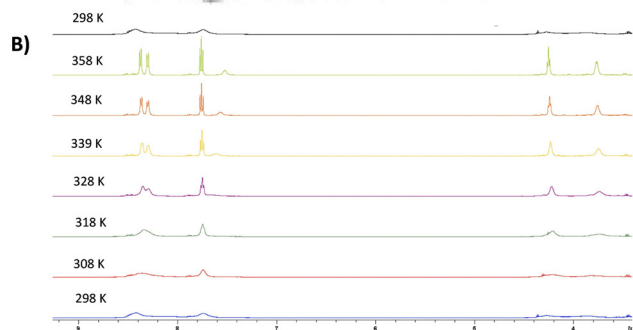
Fig. 4 Squaramides 13–15 reported by Elmes and co-workers. SEM image of 13 , and the scale bar is 10 \mu\text{m} (A). ^1\text{H-NMR} spectrum of 13 ( 5.0 \times 10^{-3} M) recorded at variable temperatures in \text{DMSO-}d_6 (B). Reproduced with permission from ref. 18. Copyright Elsevier 2022.
