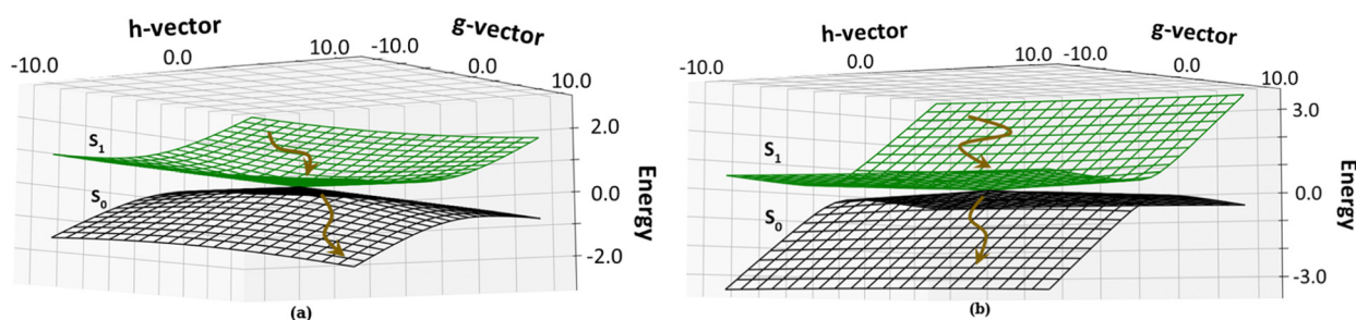
Fig. 6 Topology around the Cis: (a) Cl_1 , D ring rotated Cl and (b) Cl_2 , C-D ring rotated Cl. The deactivation of the chromophore from the S_1 state to the S_0 state is shown by brown arrows.
