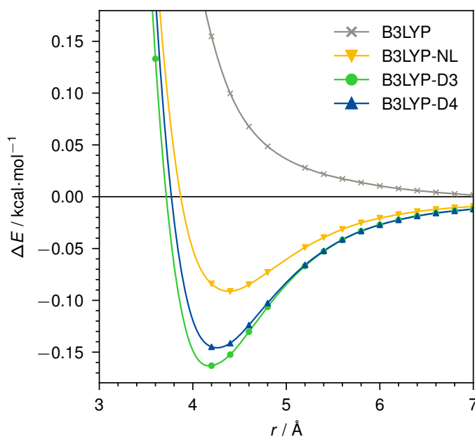
Fig. 5 Dissociation curve of \text{No—Ne} for B3LYP/def2-TZVP without dispersion correction, with NL, D3, or D4.
