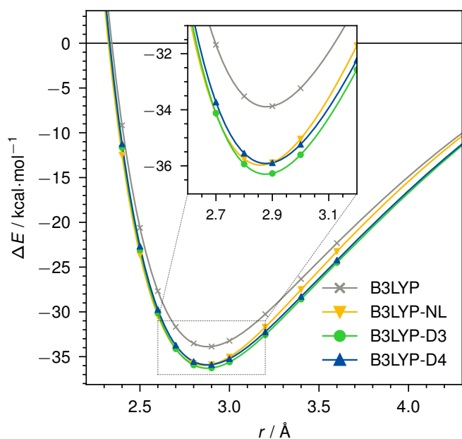
Fig. 4 Dissociation curve of \text{Ac}^{3+}\text{—Ar} for B3LYP/def2-TZVP without dispersion correction, with NL, D3, or D4.
