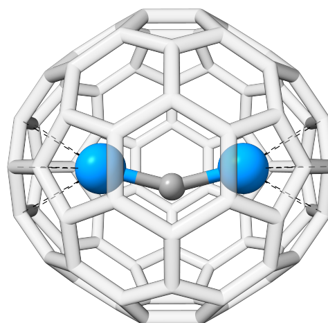
Fig. 9 PBE0-D4/def2-SVP optimized geometry of the \text{U}_2\text{C}@C_{80} -cluster.
