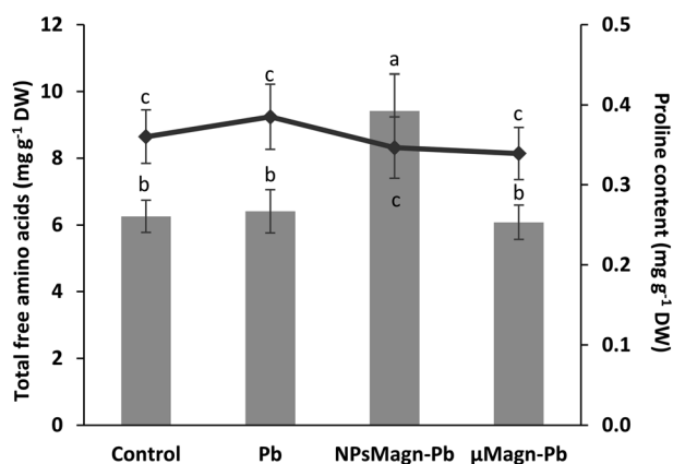
Fig. 4 Total free amino acids ( \text{mg eq leucine g}^{-1} \text{ DW} ) (histogram) and proline content ( \text{mg g}^{-1} \text{ DW} ) (curve) measured in the leaves of sunflower plants after 90 days of growth on control soil or containing Pb, NPsMgN-Pb or μMgN-Pb. Data represent the mean ± SEM ( n = 6 ). Different letters above the bars indicate significant differences ( p < 0.05 ).
