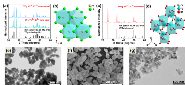
Fig. 1 Powder XRD patterns of the (a) \text{YF}_3\text{:}20\% \text{Yb}^{3+} , 2\% \text{Er}^{3+} and (c) \text{YVO}_4\text{:}20\% \text{Yb}^{3+} , 2\% \text{Er}^{3+} and (b and d) corresponding graphical representation of the arrangement of atoms in the crystal lattice, TEM/SEM images of (e) nanocrystalline \text{YF}_3\text{:Yb}^{3+} , \text{Er}^{3+} , (f) microcrystalline \text{YF}_3\text{:Yb}^{3+} , \text{Er}^{3+} , and (g) nanocrystalline \text{YVO}_4\text{:Yb}^{3+} , \text{Er}^{3+} .
