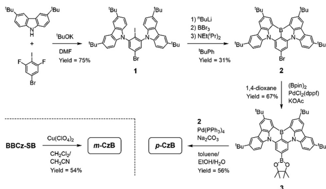
Scheme 1 Synthetic Routes to p-CzB and m-CzB .
