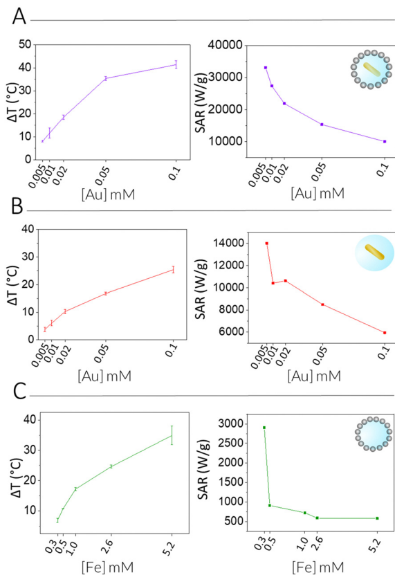
Fig. 3 Average PTH temperature increase ( \Delta T , °C) and estimated SAR, using conditions of 5 min irradiation (808 nm) at 2.5 \text{ W cm}^{-2} in solution, at different concentrations of AuNR@SiO 2 @IONPs (A), AuNR@SiO 2 (B), and SiO 2 @IONPs (C). Results show mean \pm SD of triplicate measurements (error bars for SAR are within the symbols).
