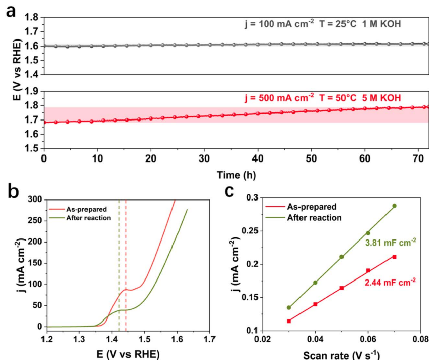
Fig. 2 Electrochemical characterization of FeNiCr/FF under industrially relevant conditions. (a) Long-term OER stability performance of FeNiCr/FF under standard and simulated industrial conditions. (b) Polarization curves and (c) double-layer capacitance in comparison with the as-prepared electrode.
