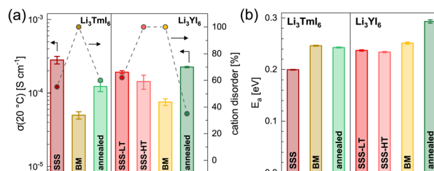
Fig. 3 Comparison of the ionic transport properties obtained from EIS for \text{Li}_3\text{TmI}_6 and \text{Li}_3\text{YI}_6 synthesized via SSS, MCBM without and with subsequent calcination. Ionic conductivities at 20^\circ\text{C} and degree of intra-layer cation disorder in (a) and activation energy for ion diffusion are depicted in (b).
