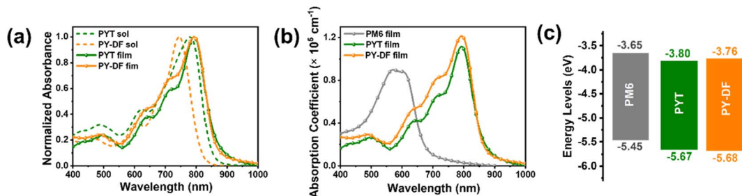
Fig. 2 (a) Normalized UV-vis-NIR absorption spectra of PYT and PY-DF in solution and as thin films. (b) Absorption coefficient of PM6, PYT and PY-DF films. (c) Energy level diagram of PM6, PYT, and PY-DF.
