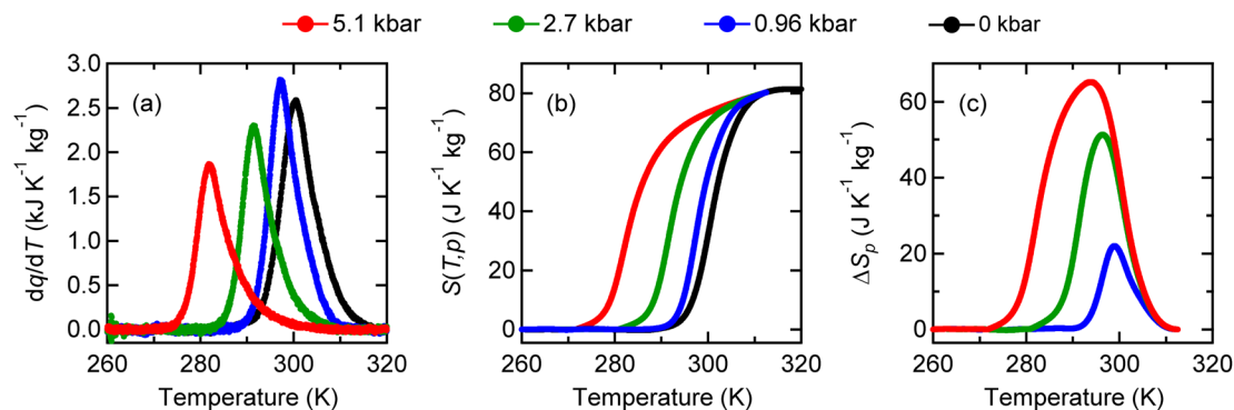
Fig. 2 (a) Heat flow curves divided by the cooling rate dq/dT , (b) corresponding entropy as a function of temperature, and (c) isothermal entropy changes of NdCu 3 Fe 4 O 12 under various applied pressures.
