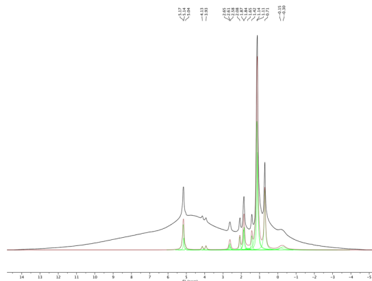
Fig. 10 ^1\text{H} MAS NMR and deconvoluted spectra of pure sHAP (2Q: 15 \mu\text{L} \text{g}^{-1} Neutrased, 7.5 \mu\text{L} \text{g}^{-1} Lipozyme CALB L, 6 h, 40 ^\circ\text{C} ).
