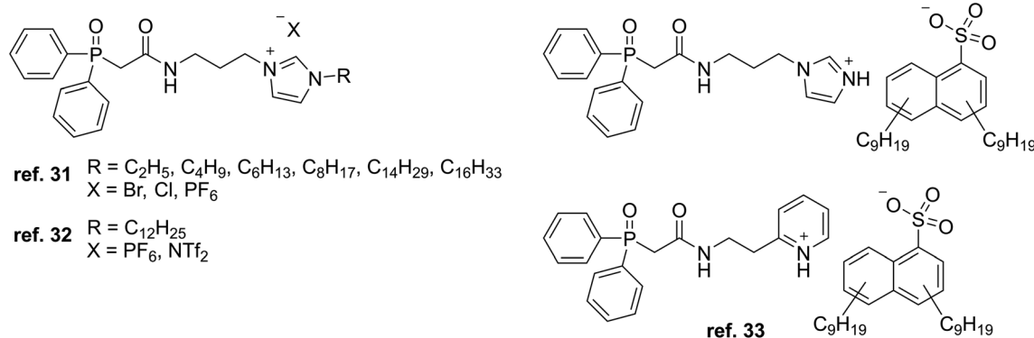
Fig. 4 CMPO-based TSILs.
