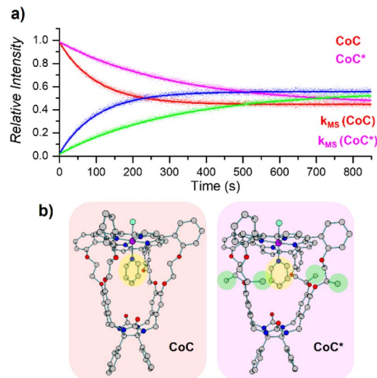
Fig. 6 (a) Relative time evolution of [\text{CoC}(\text{Py})]^+ (red), [\text{CoC}(\text{Py})]^+ (blue), [\text{CoC}^*(\text{Py})]^+ (magenta), and [\text{CoC}^*(\text{Py})]^+ (green) in a single DRL experiment carried out at 40 °C in \text{CHCl}_3 with 200 equiv. pyridine and 200 equiv. pyridine-D5. Dots are experimental data points, and lines correspond to fittings of experimental data by eqn (S1) and (S2).† (b) DFT-calculated structures of ^1[\text{CoC}(\text{Cl}_{\text{OUT}})(\text{Py}_{\text{IN}})] and ^1[\text{CoC}^*(\text{Cl}_{\text{OUT}})(\text{Py}_{\text{IN}})] optimized with B3LYP-D3/def2svp.
